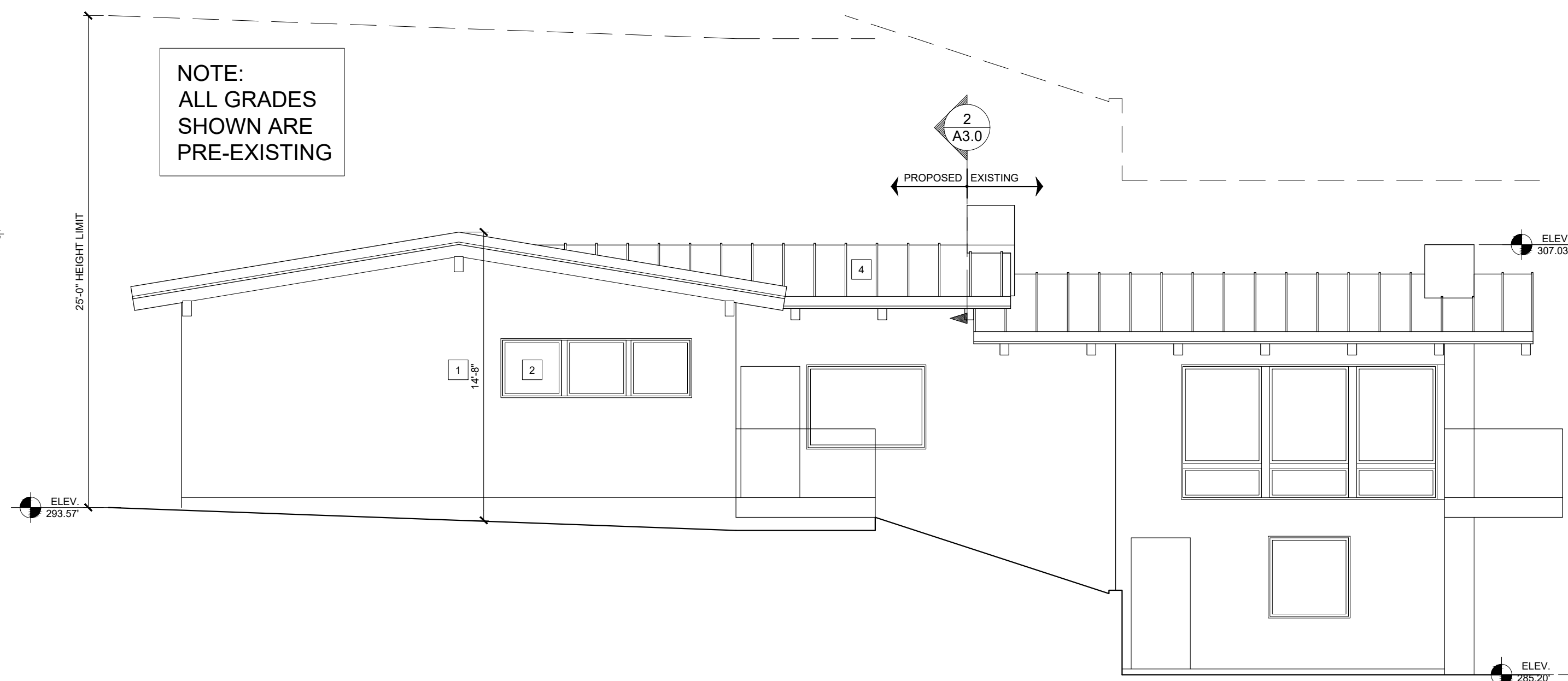
NORTHWEST
