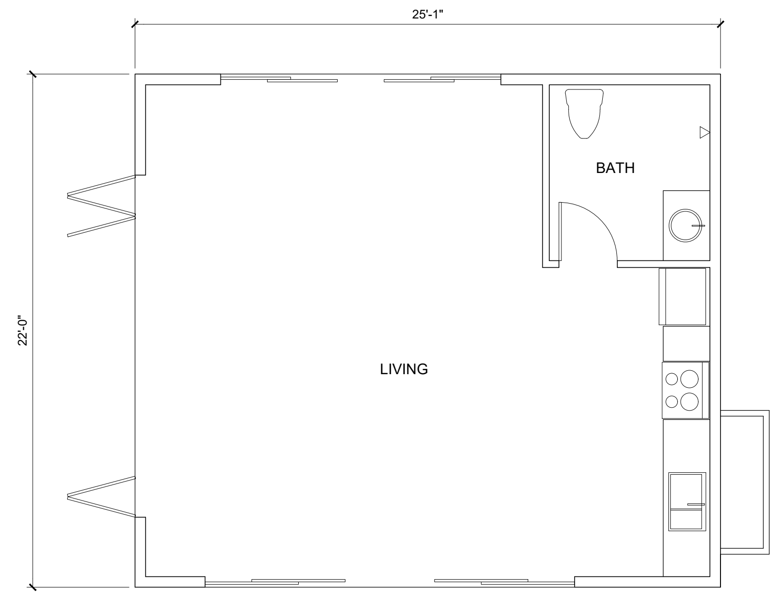
ADU FLOOR PLAN
