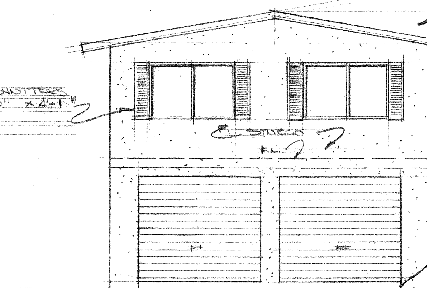
FRONT
