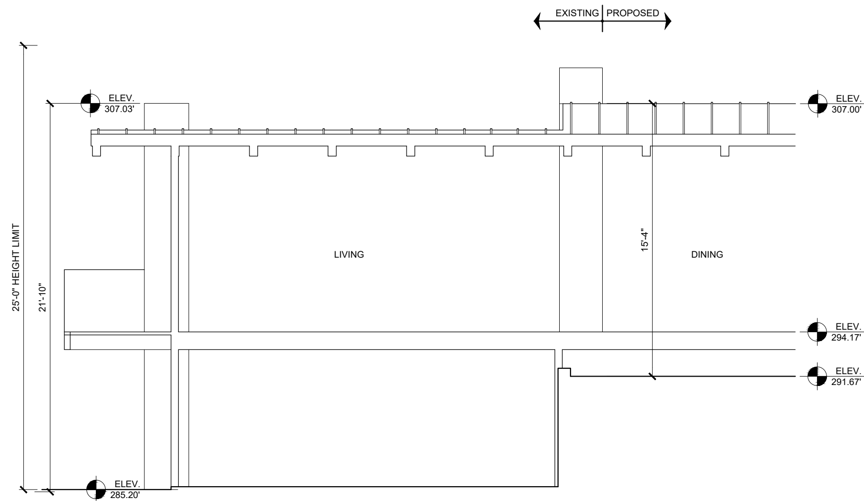
SECTION 1
