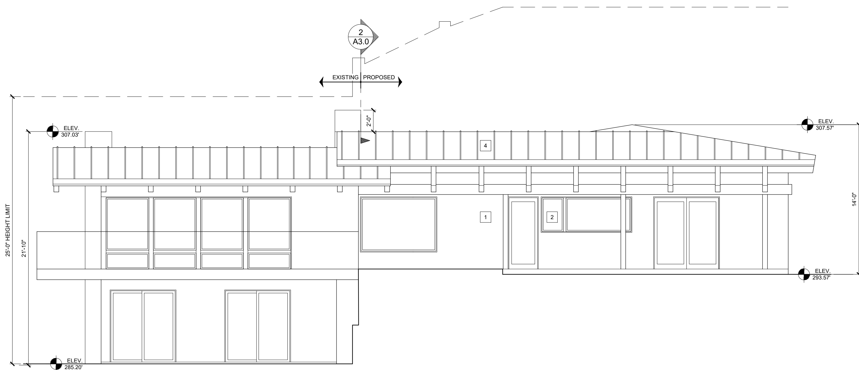
SOUTHEAST
