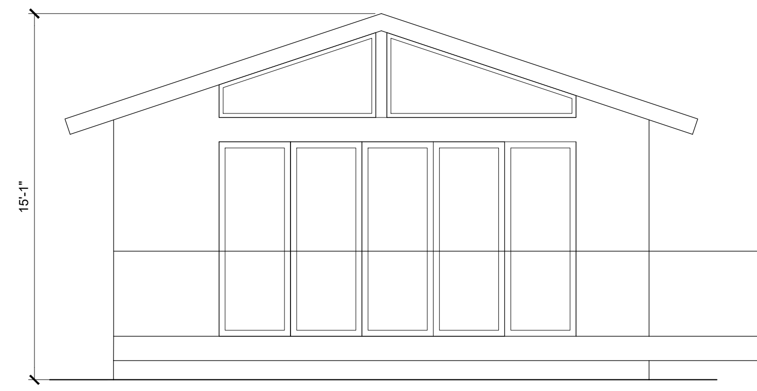
ADU SOUTHWEST 1/4" = 1'-0"
