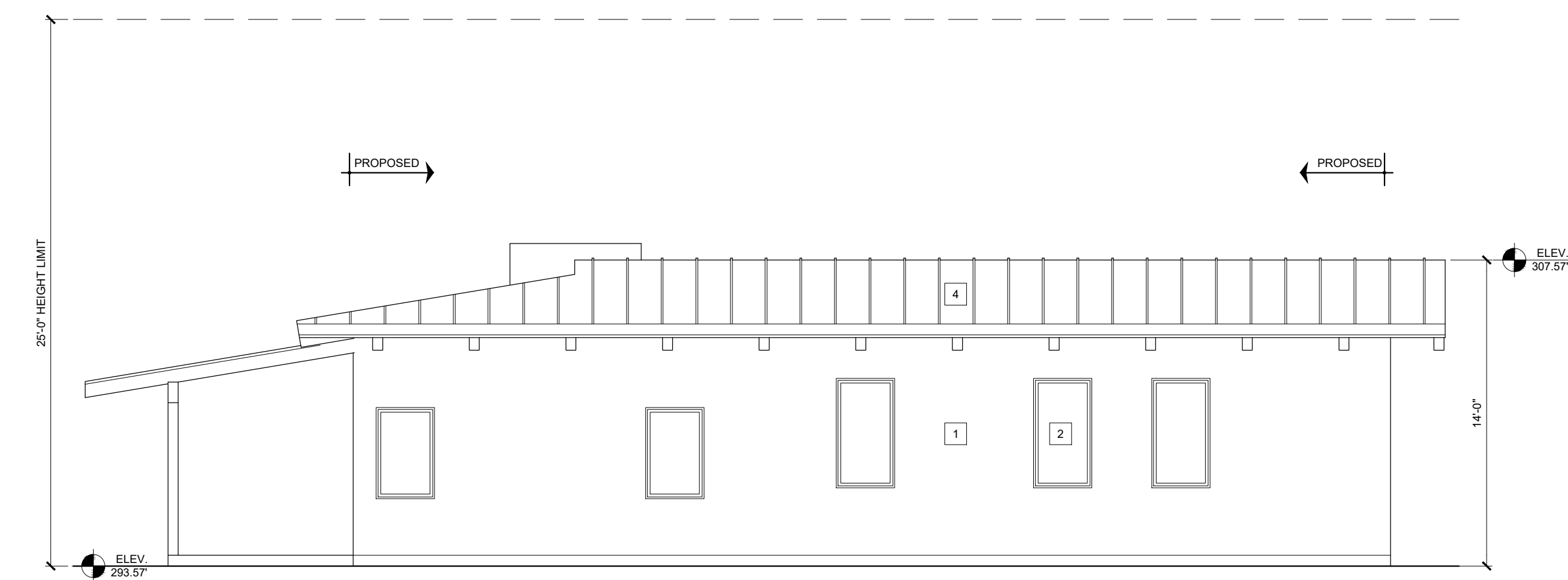
NORTHEAST
