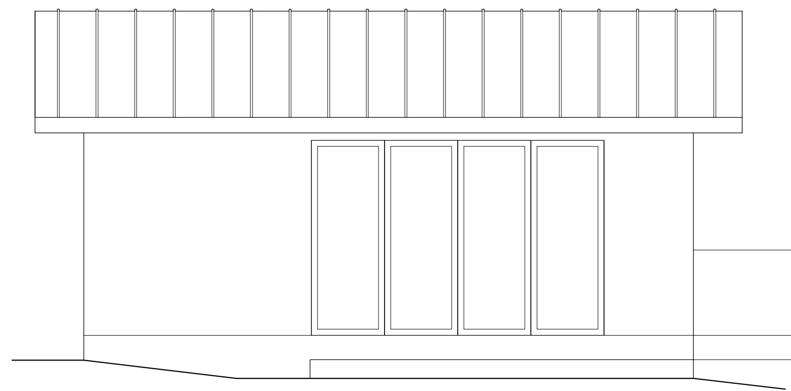
ADU NORTHWEST 1/4" = 1'-0"
