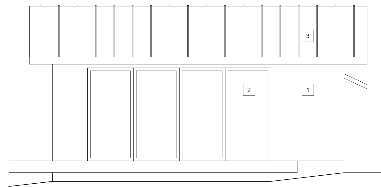
ADU SOUTHEAST 1/4" = 1'-0"
