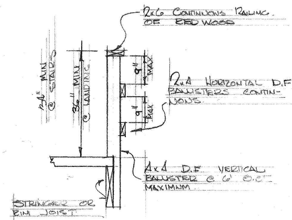
TYPICAL RAIL DETAIL FOR LANDING & STAIRS NO SCALE
