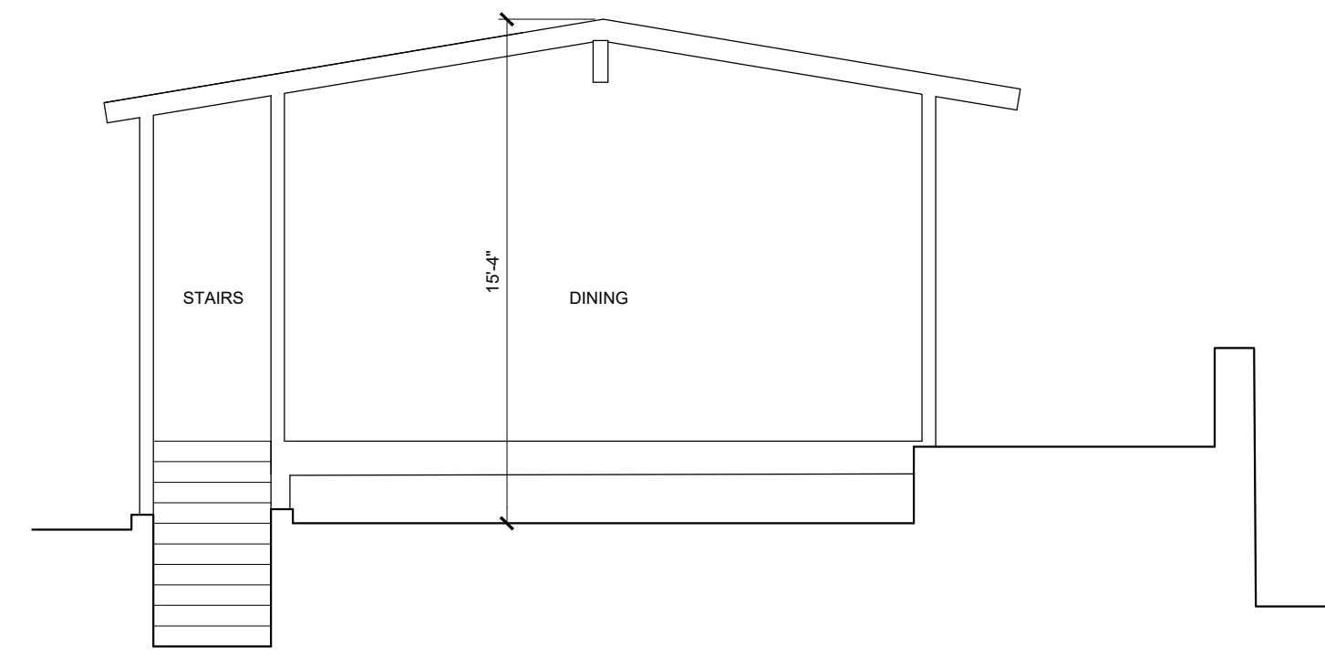
SECTION 2
