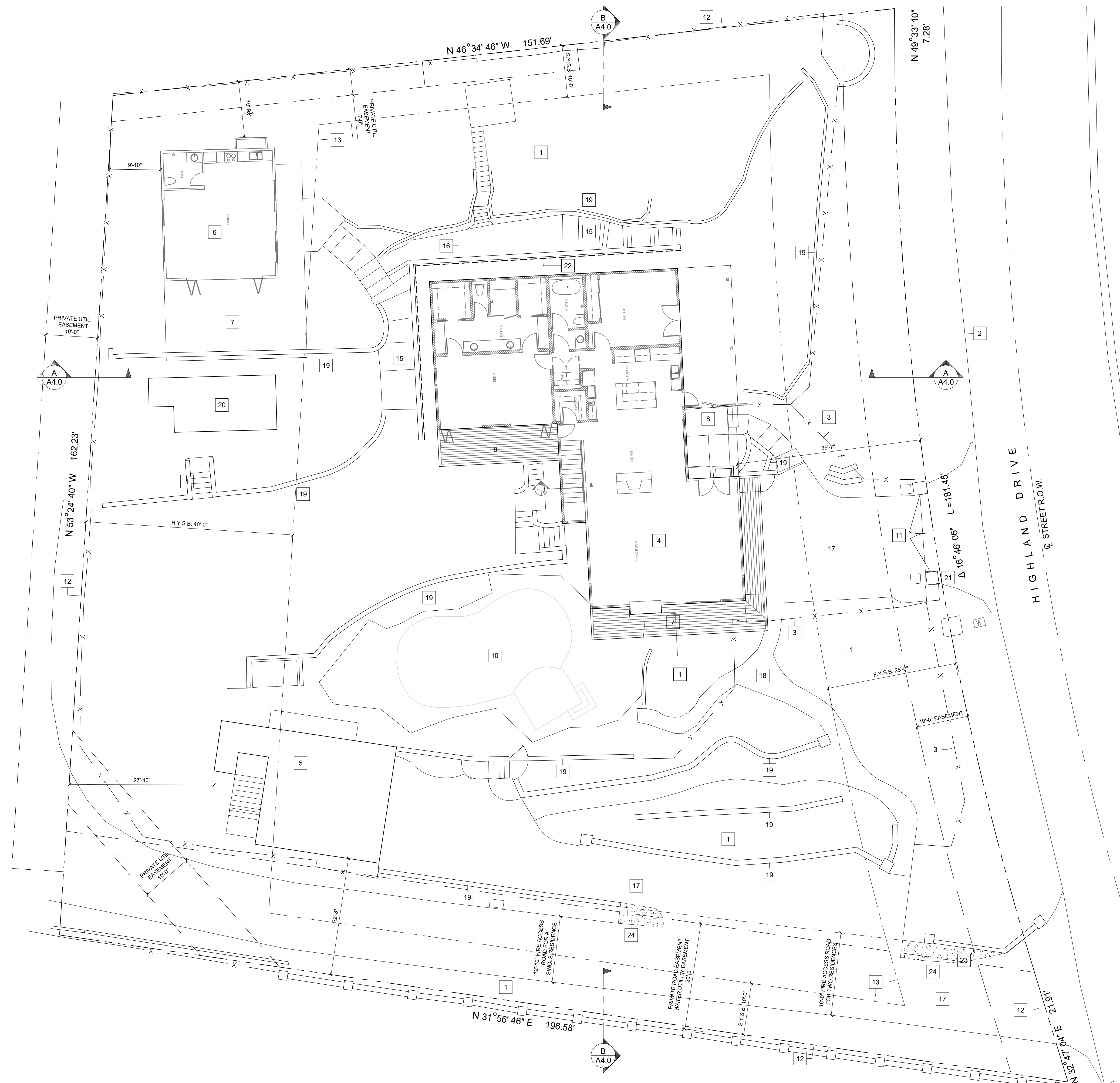
PROPOSED SITE PLAN SCALE: 1/10" = 1'-0"
