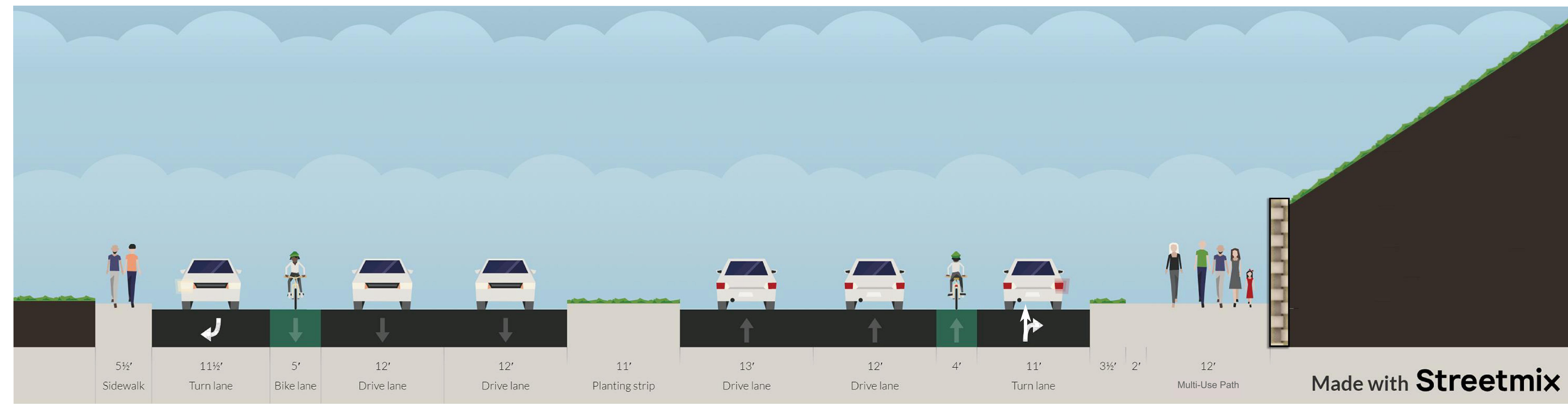
SECTION E-E: PROPOSED
