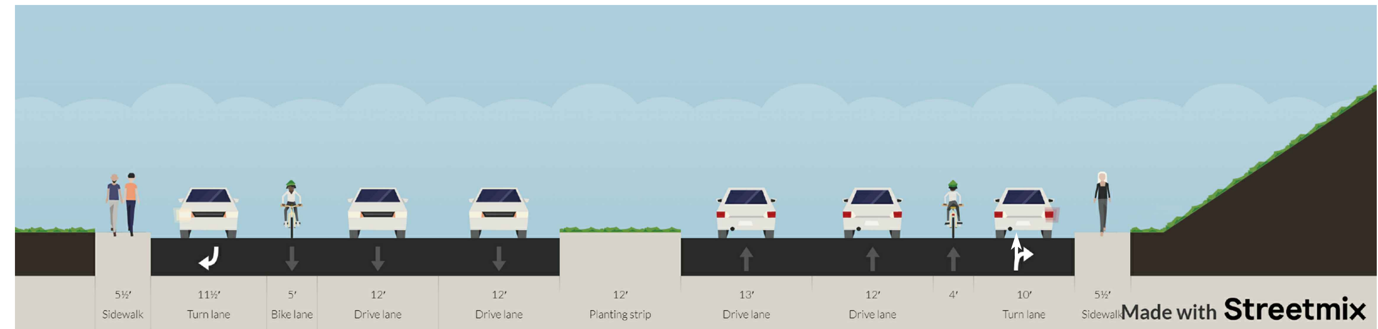
SECTION E-E: EXISTING
